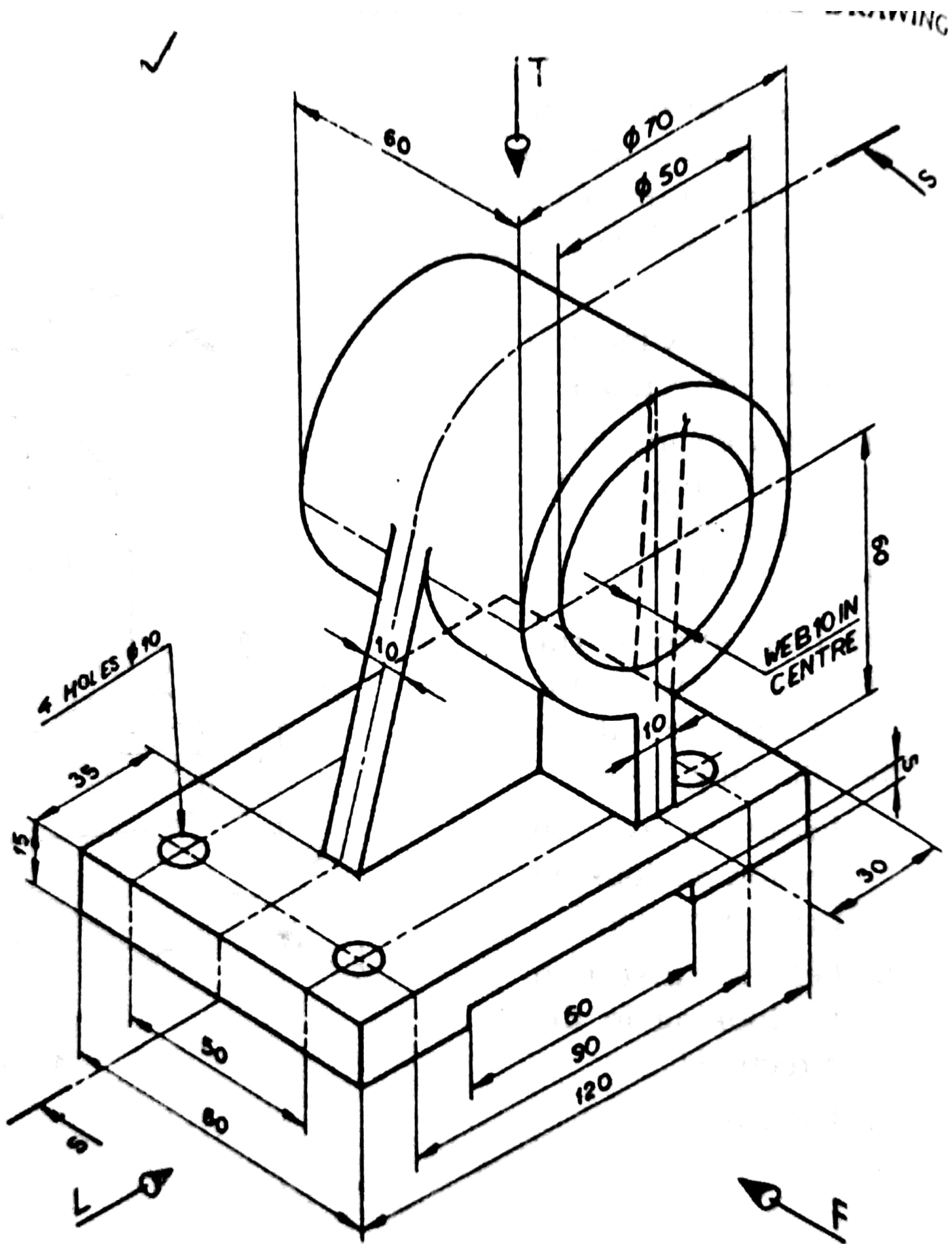
All Dimensions in mm Fig. 3.45
